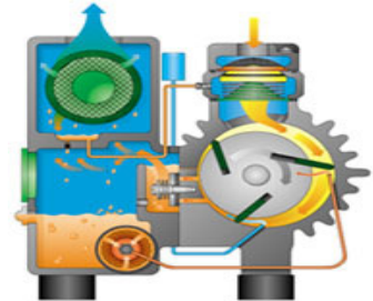
ROTARY VANE PUMPS
